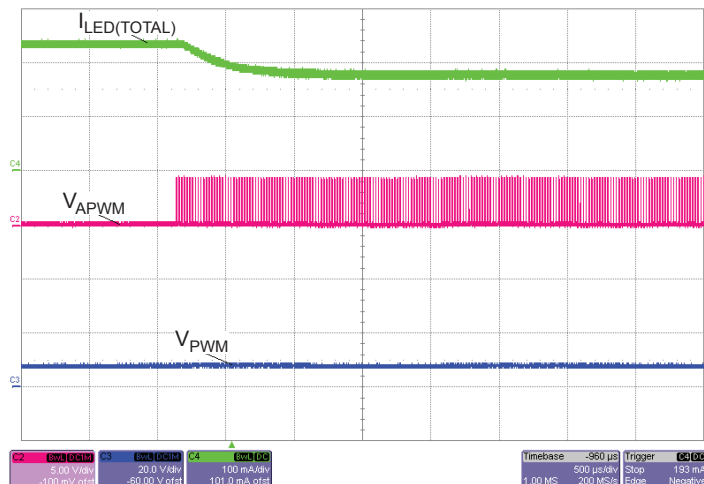
Figure 15: Transition of total LED current from 240 mA to 180 mA, when a 50 kHz 25% APWM signal is applied to the APWM pin. (Dimming PWM = 100%)
