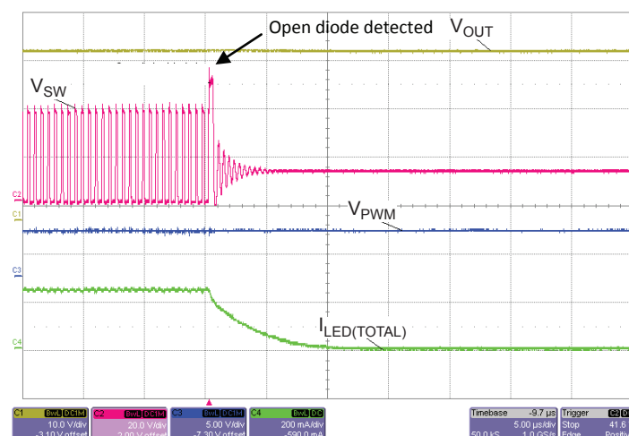
Figure 23: Open Schottky Diode Protection
