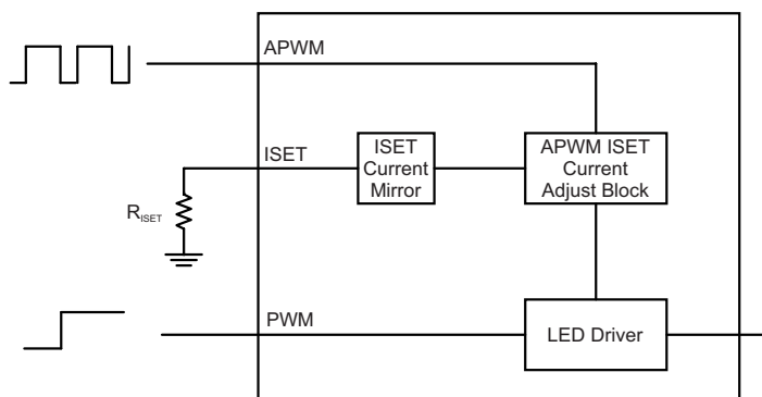
Figure 12: Simplified Block Diagram of APWM ISET Block
