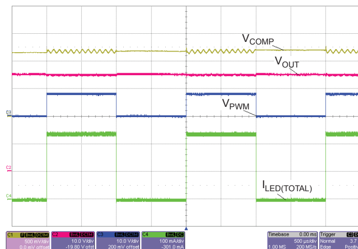
Figure 8: Typical PWM Diagram Showing V_{OUT} , I_{LED} , and COMP Pins, as well as the PWM Signal. (PWM dimming Frequency is 500 Hz 50% duty cycle.)
