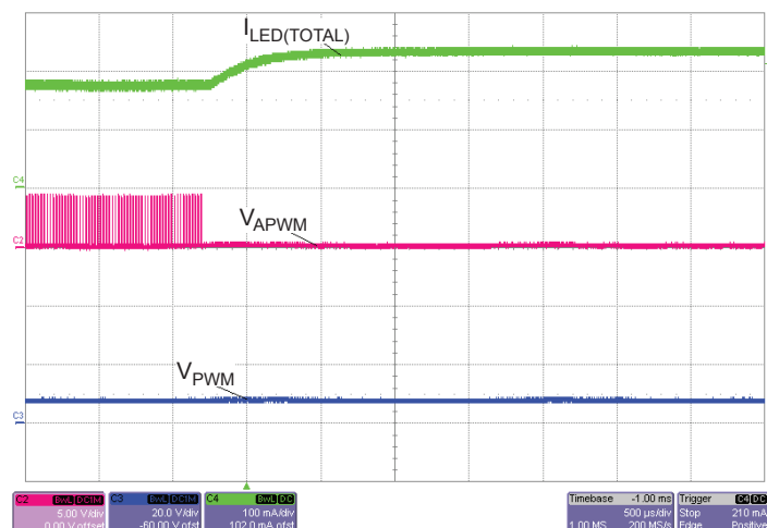
Figure 16: Transition of total LED current from 180 mA to 240 mA, when a 50 kHz 25% APWM stops being applied to the APWM pin. (Dimming PWM = 100%)
