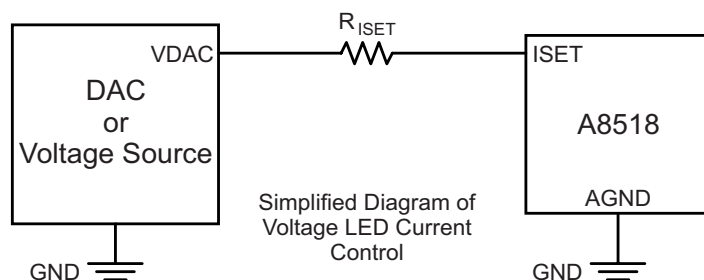
Figure 18: Typical Application Circuit Using a DAC to Control the LED Current in the A8518
