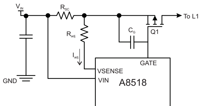
Figure 27: Typical Circuit Showing Implementation of Input Disconnect Feature
