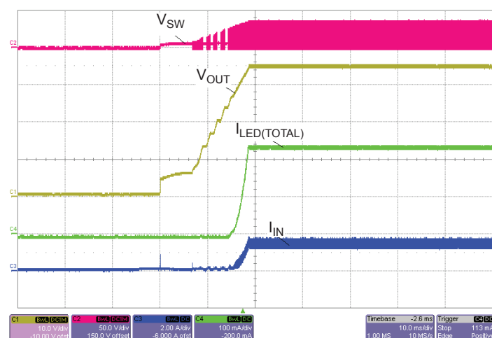
Figure 7: Startup Diagram Showing the Input Current, Output Voltage, Total LED Current, and Switch Node Voltage
