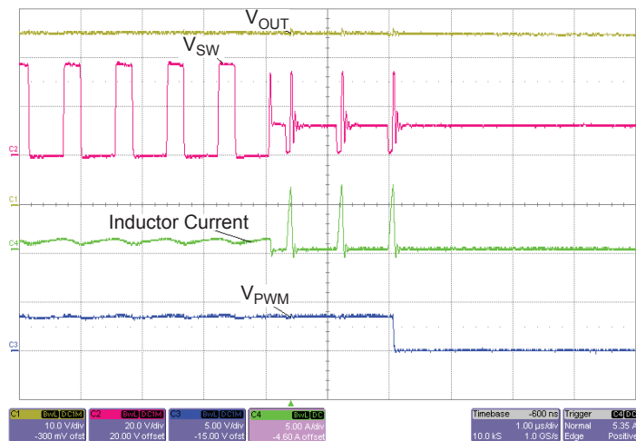
Figure 26: Secondary Boost Switch OCP
