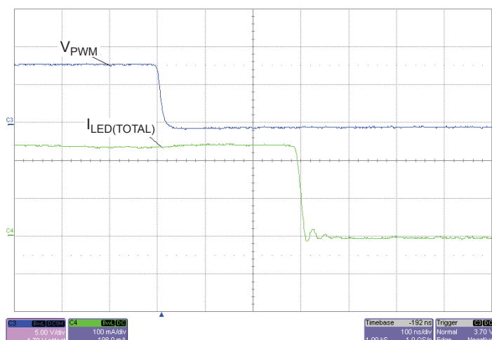
Figure 11: Falling Edge PWM Signal to Total LED Current I_{LED(TOTAL)} Turn-Off Delay. Time base = 100 ns
