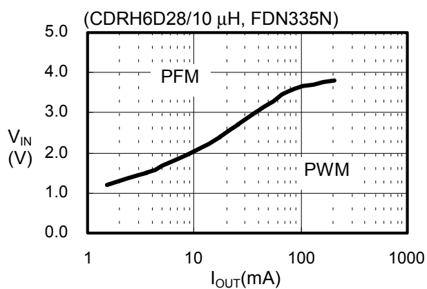
(35) S-8341C50AFT
