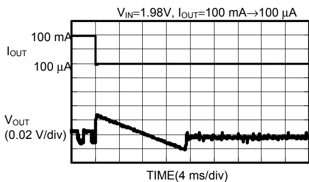
(2) S-8340A33AFT, fosc=600 kHz
