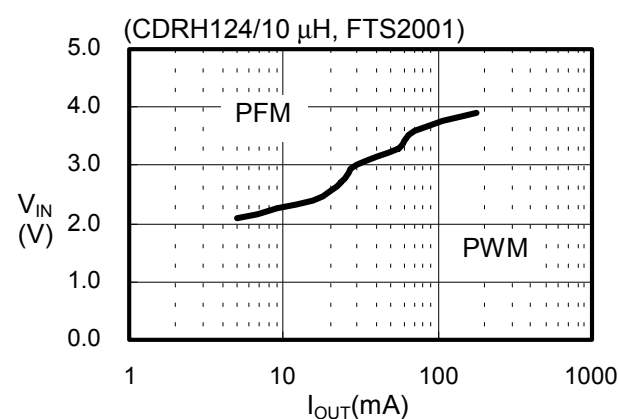
(36) S-8341C50AFT
