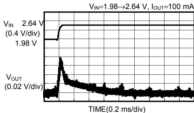
S-8340C33AFT, fosc=300kHz
