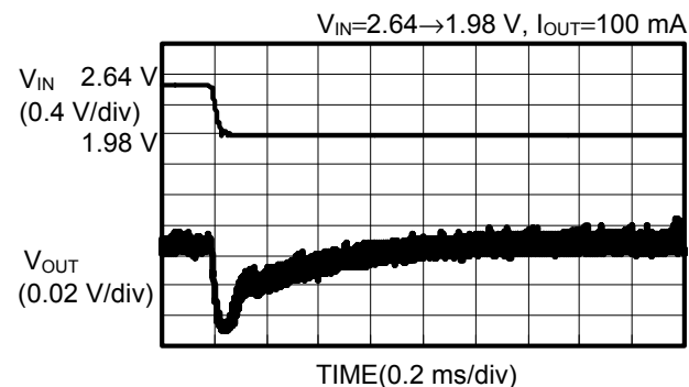
S-8340C33AFT, fosc=300kHz
