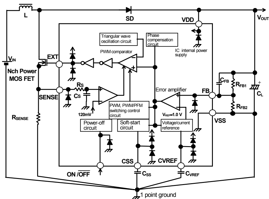
Figure 11 Block diagram <Output voltage external setting type>
