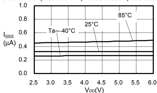
S-8340A33A(fosc:600 kHz) / S-8340C33A(fosc:300 kHz)
