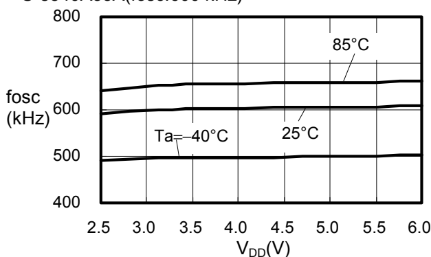
S-8340A33A(fosc:600 kHz)
