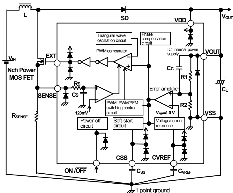
Figure 10 Block diagram <Output voltage fixed output type>
