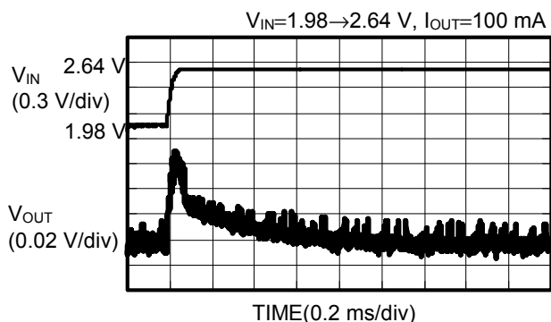
(1) S-8340A33AFT, fosc=600kHz
