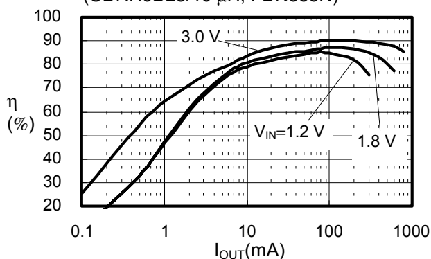
(19) S-8341C33AFT
