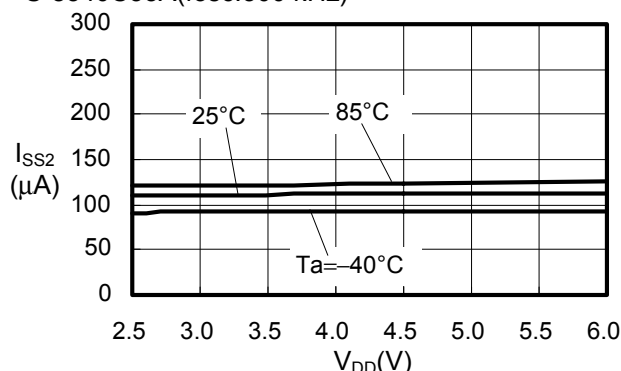
S-8340C33A(fosc:300 kHz)
