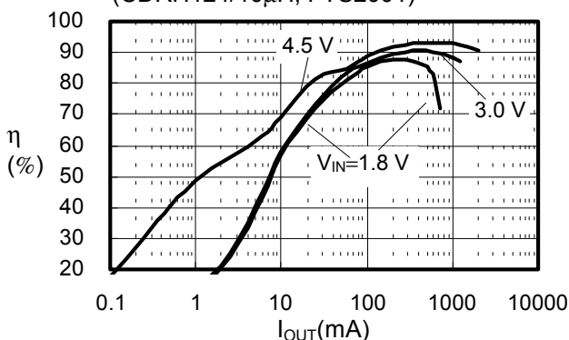
(24) S-8341C50AFT
