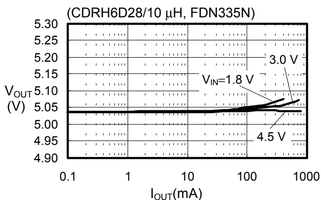
(23) S-8341C50AFT
