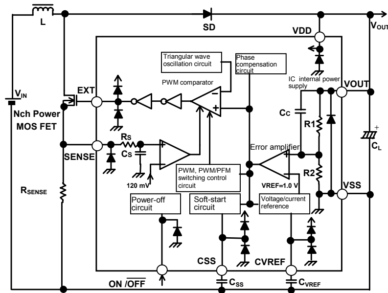
Figure 1 Block diagram <Output voltage fixed output type>
