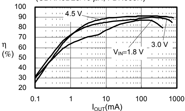
(23) S-8341C50AFT
