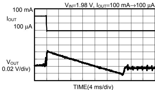
S-8340C33AFT, fosc=300 kHz
