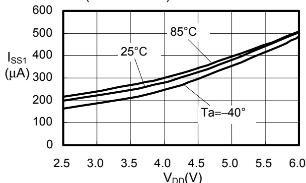
S-8340C33A(fosc:300 kHz)
