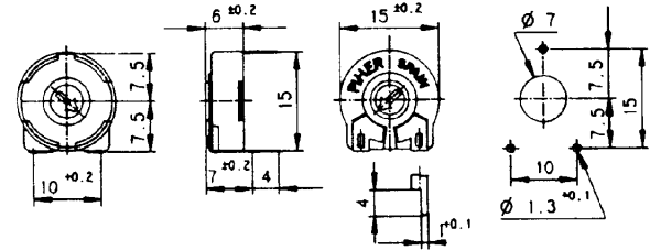
PT 15 Lv (15) PTC 15 Lv (15)
