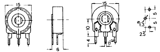
PT15 NGh (2,5) PTC15 NGh (2,5)
