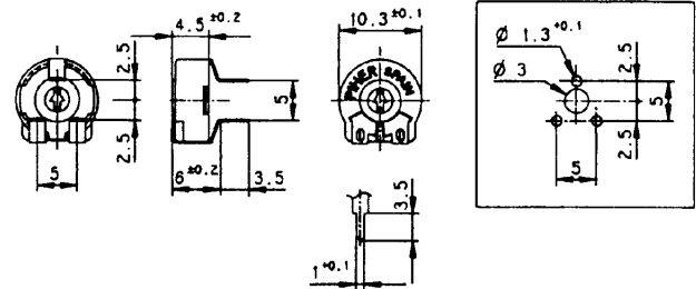
PT 10 Lv (5) PTC 10 Lv (5)
