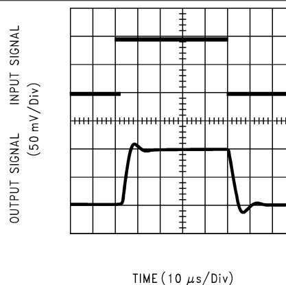
Figure 5-16. Inverting Small-Signal Pulse Response
