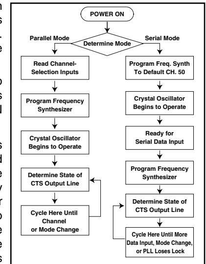
Figure 10: Start-up Sequence
