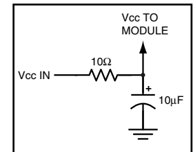
Figure 11: Supply Filter
