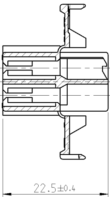
Section A-A SECTION
