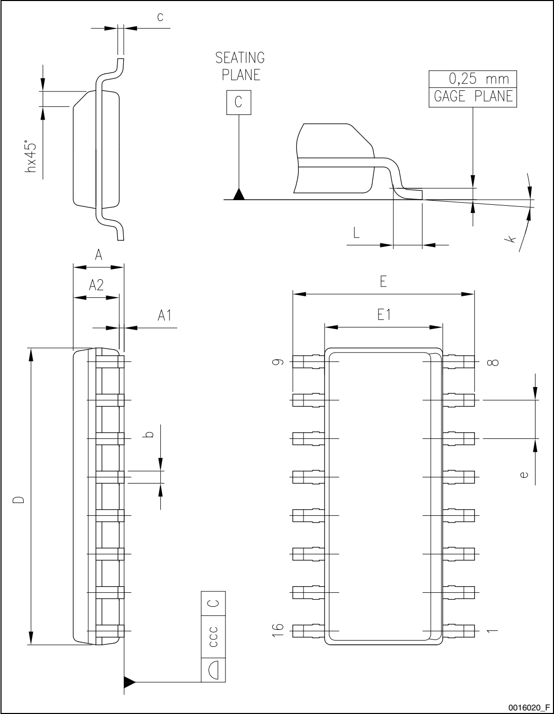
Figure 25. SO16N drawing
