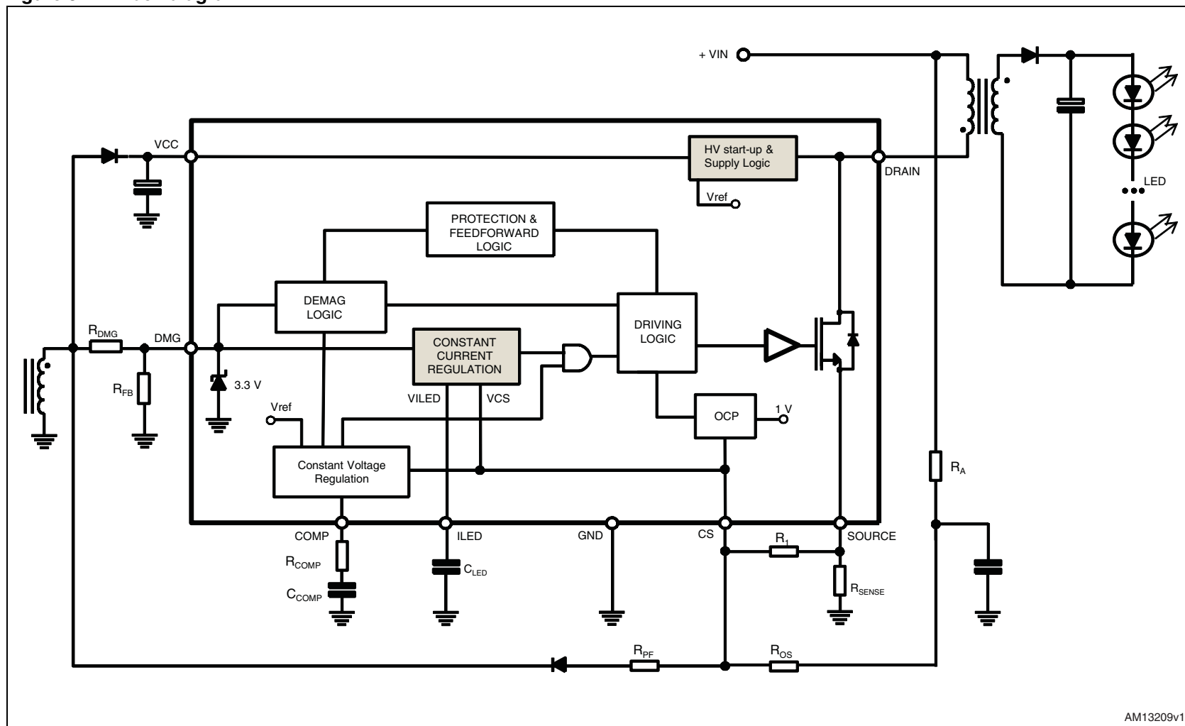
Figure 3. Block diagram
