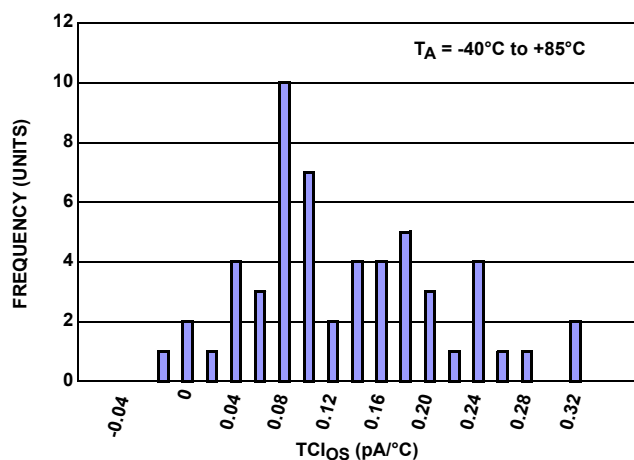
FIGURE 32. TCI_{OS} HISTOGRAM
