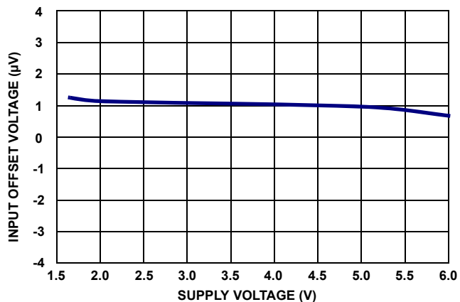
FIGURE 1. V_{OS} vs SUPPLY VOLTAGE
