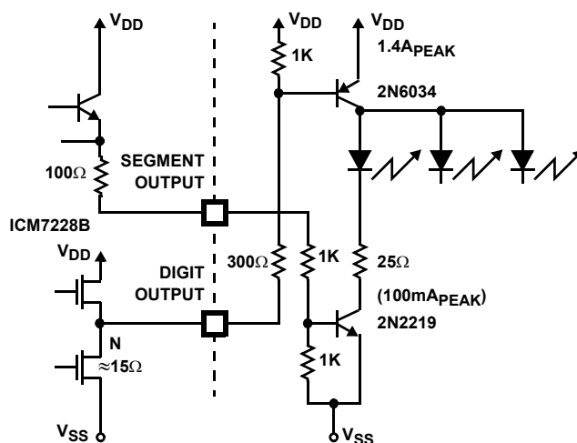
FIGURE 16. DRIVING HIGH CURRENT DISPLAY, COMMON CATHODE ICM7228B TO COMMON ANODE DISPLAY
