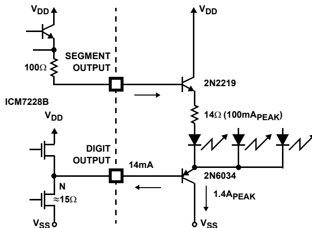
FIGURE 15. DRIVING HIGH CURRENT DISPLAY, COMMON CATHODE ICM7228B TO COMMON CATHODE DISPLAY
