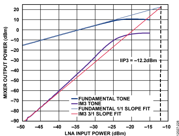
Figure 17. LNA/Mixer IIP3, V_{DD} = 3.0\text{ V} , Temperature = 25^{\circ}\text{C} , RF = 915 MHz, LNA Gain = High, Mixer Gain = High, Source 1 Frequency = 915 MHz + 0.4 MHz, Source 2 Frequency = 915 MHz + 0.7 MHz
