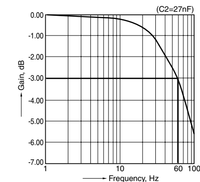
5. Frequency characteristics
