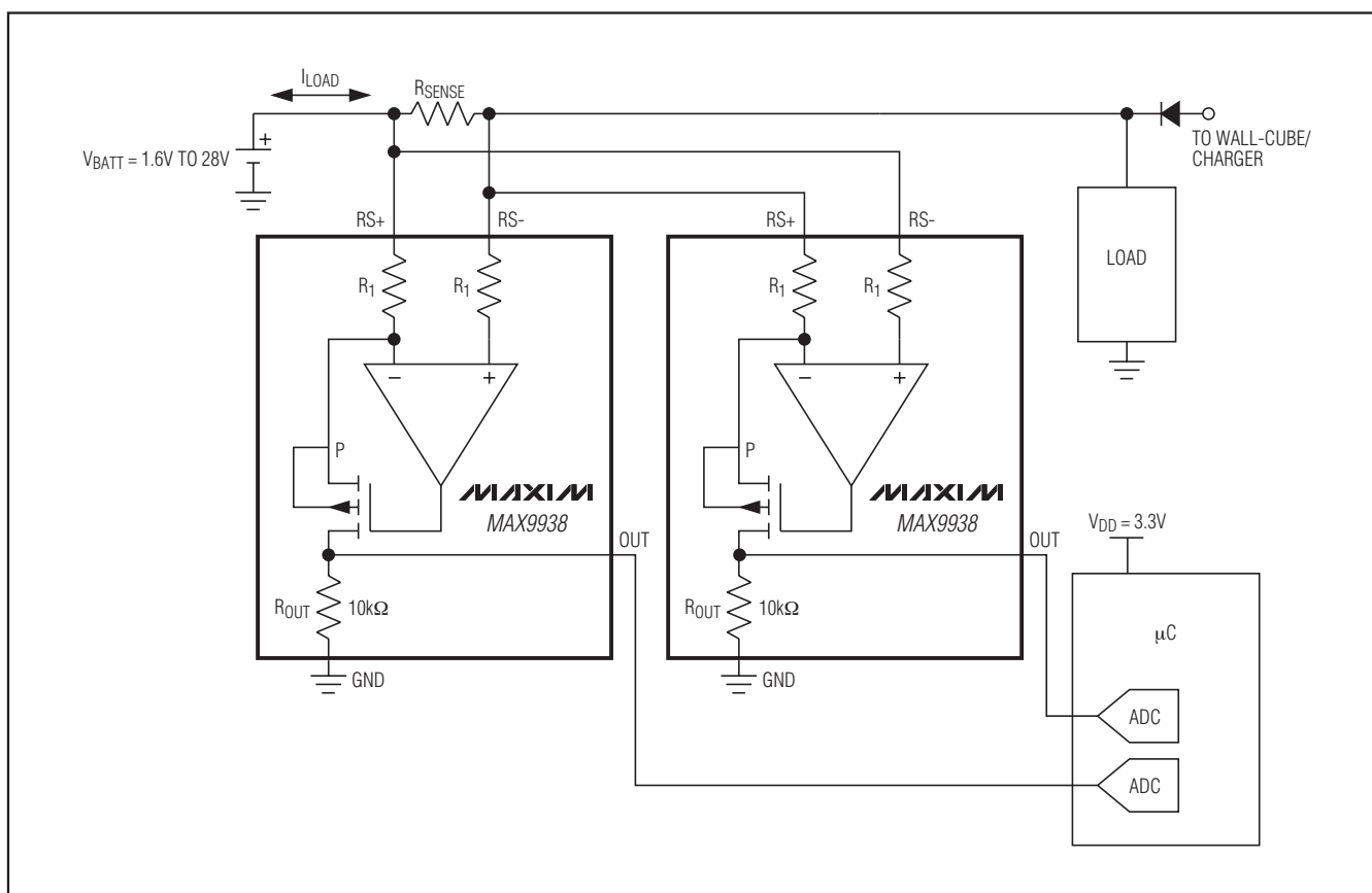
Figure 3. Bidirectional Application
