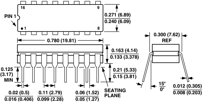
16-Lead Cerdip (Q-16)
