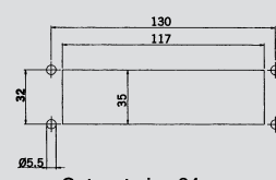
Cut-out size 24 35 x 117 mm
