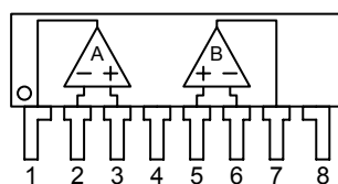
NJM2100L
