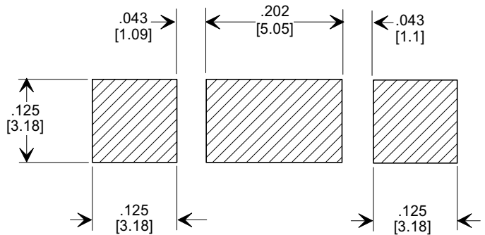
SUGGESTED MOUNTING PATTERN (SCALE 5 X)
