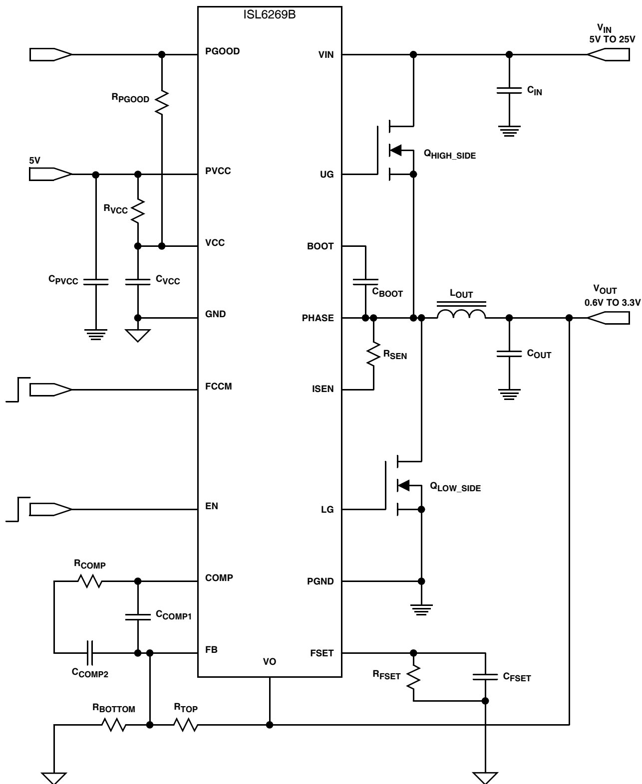
FIGURE 2. ISL6269B TYPICAL APPLICATION SCHEMATIC
