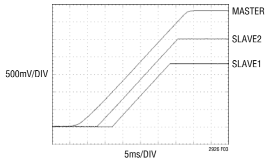
Figure 3. Offset Tracking
