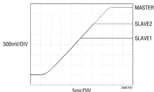
Figure 1. Coincident Tracking
