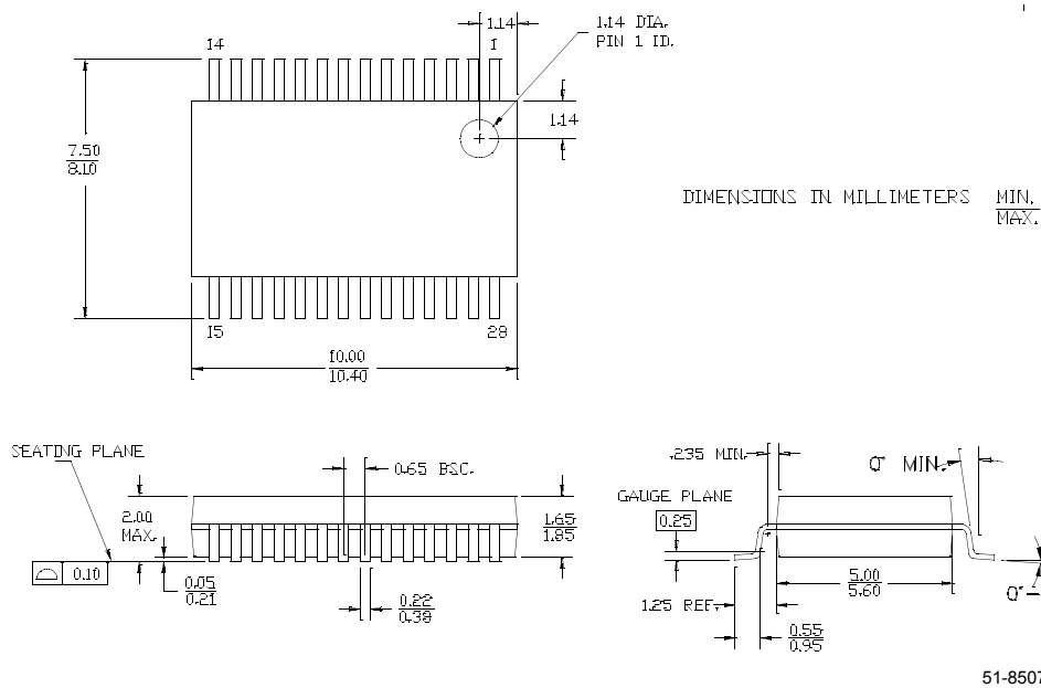
Figure 22. 28-Pin (210-Mil) SSOP
