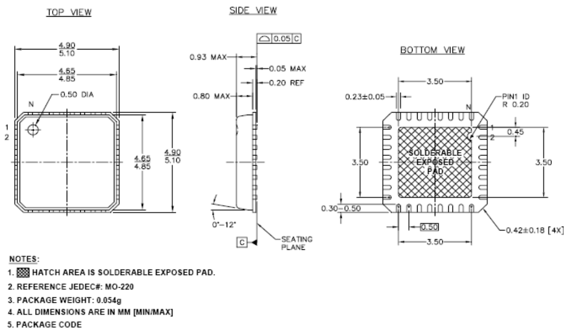
Figure 24. 32-Pin (5x5 mm) QFN
