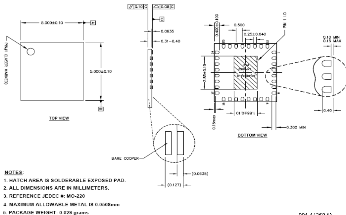
Figure 25. 32-Pin (5 X 5 X 0.4MM) QFN (SAWN 1.85 X 2.85) EPAD
