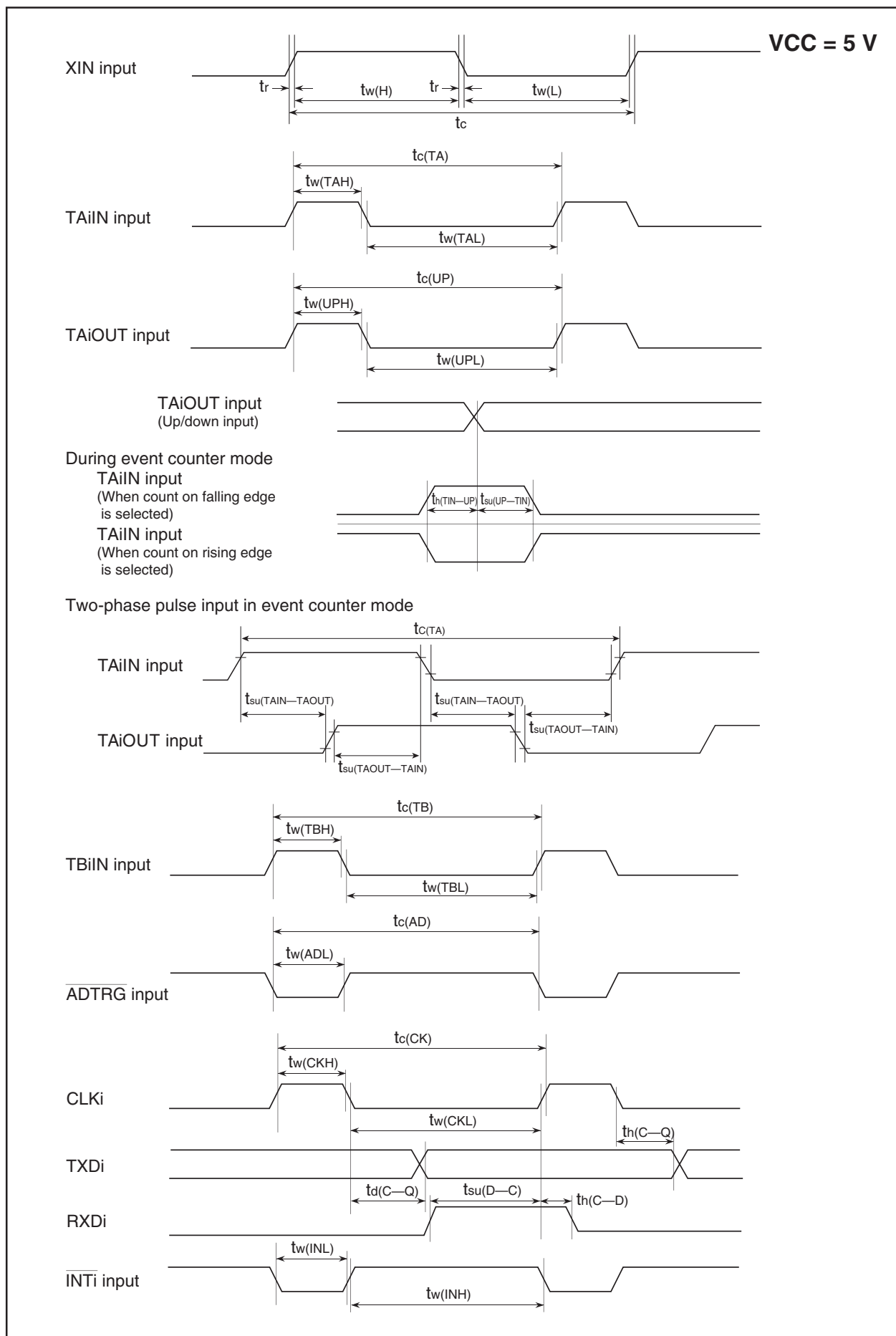
Figure 5.13 Timing Diagram (1)
