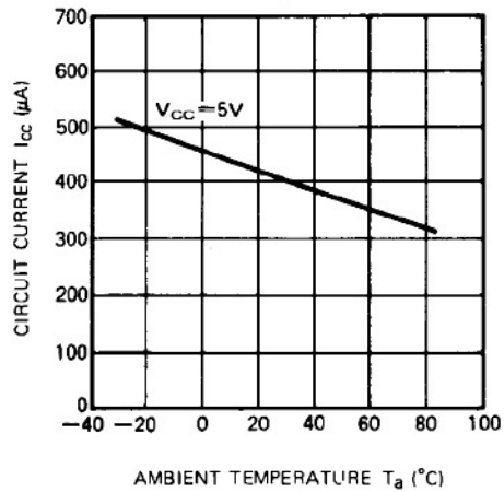
CIRCUIT CURRENT VS. AMBIENT TEMPERATURE (M51953B, M51954B)
