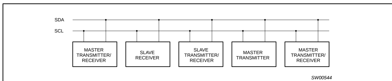
Figure 16. System configuration
