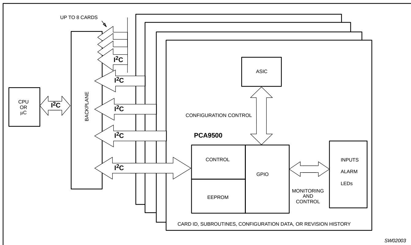
Figure 18. Typical application
