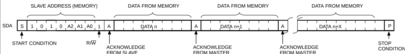
Figure 13. Sequential Read
