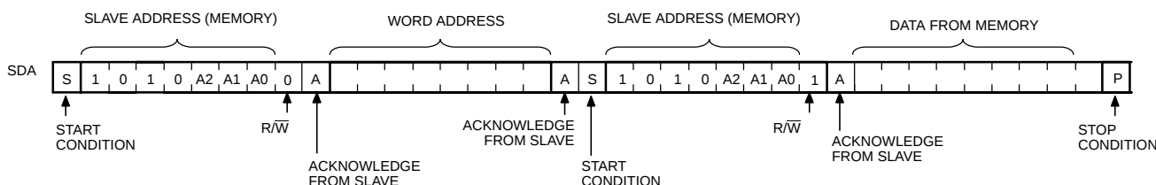
Figure 12. Random Read
