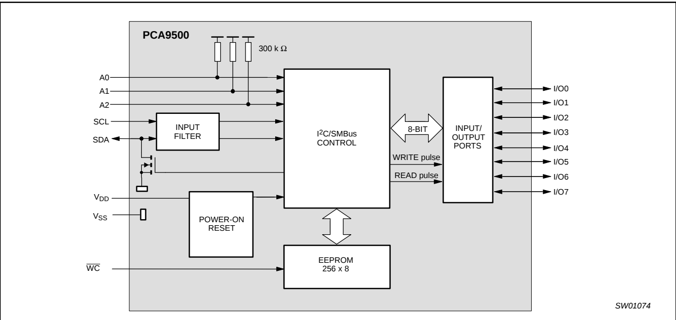
Figure 3. Block diagram
