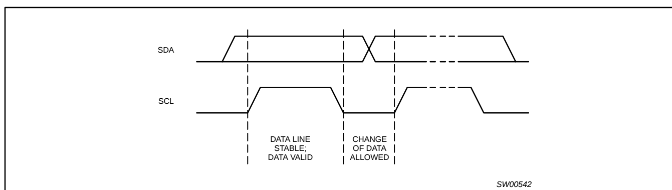
Figure 14. Bit transfer
