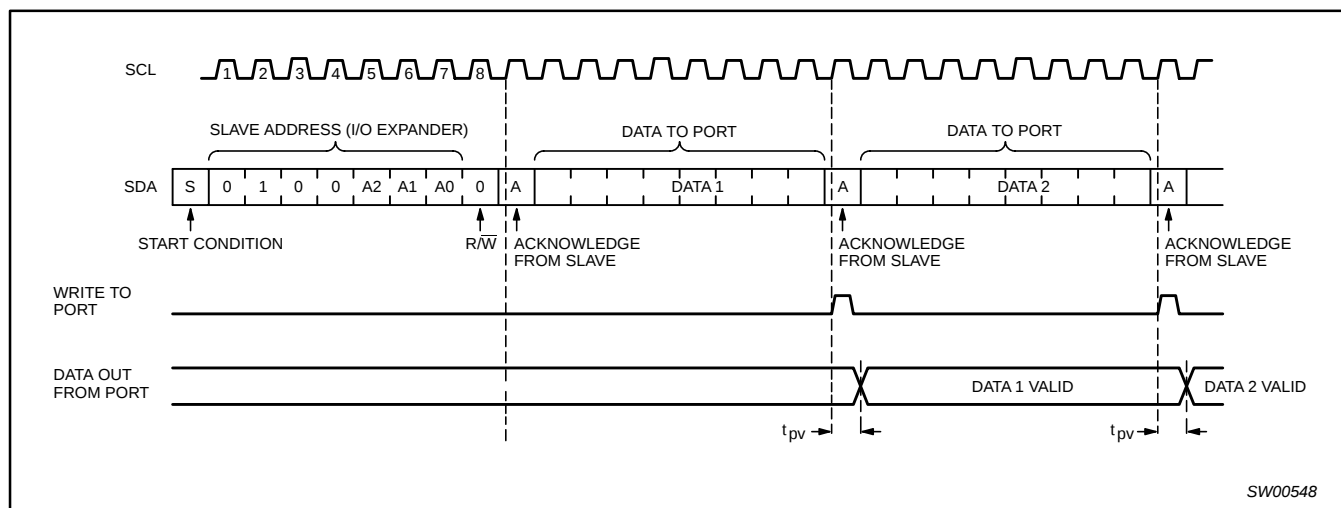
Figure 6. I/O WRITE mode (output)
