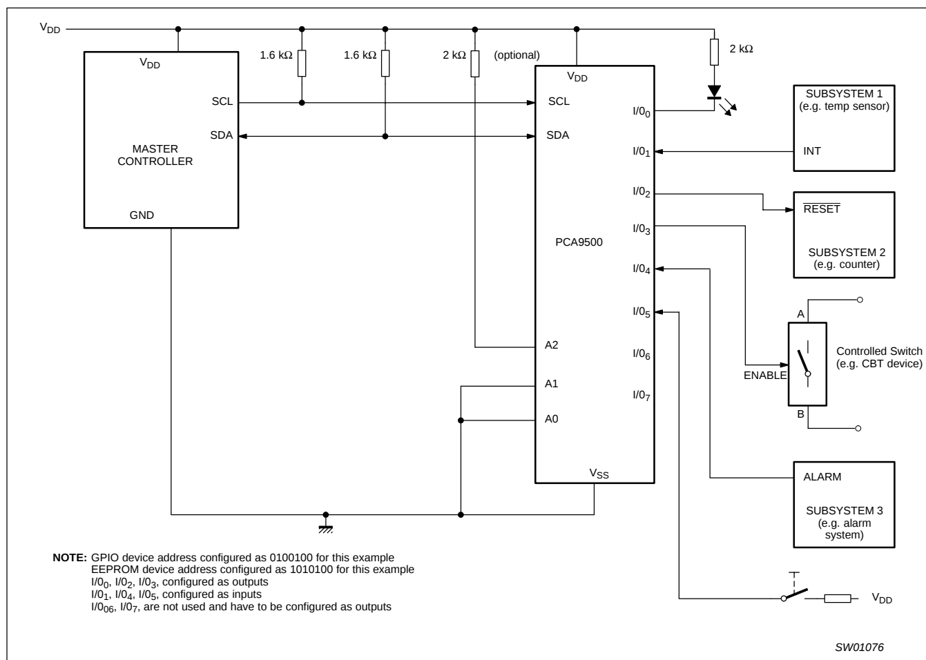
Figure 19. Typical application
