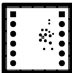
Figure 9. SMP-TPS7A4001-MVK Board Solder Mask – Bottom Side
