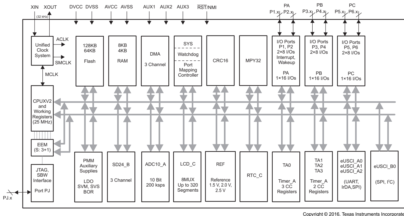
Figure 6-2. Functional Block Diagram – PN Package
