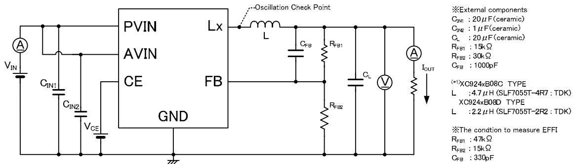
1) CIRCUIT ①
