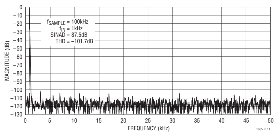
Figure 11. LTC1605 Nonaveraged 4096 Point FFT Plot
