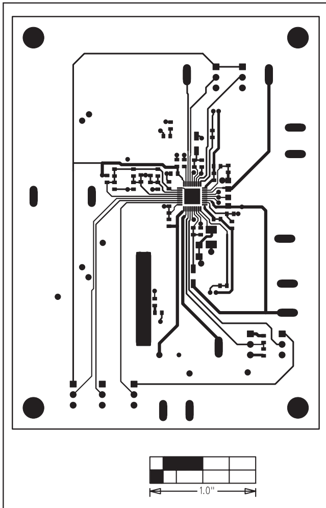
Figure 6. MAX1537 EV Kit PC Board Layout—Solder Side
