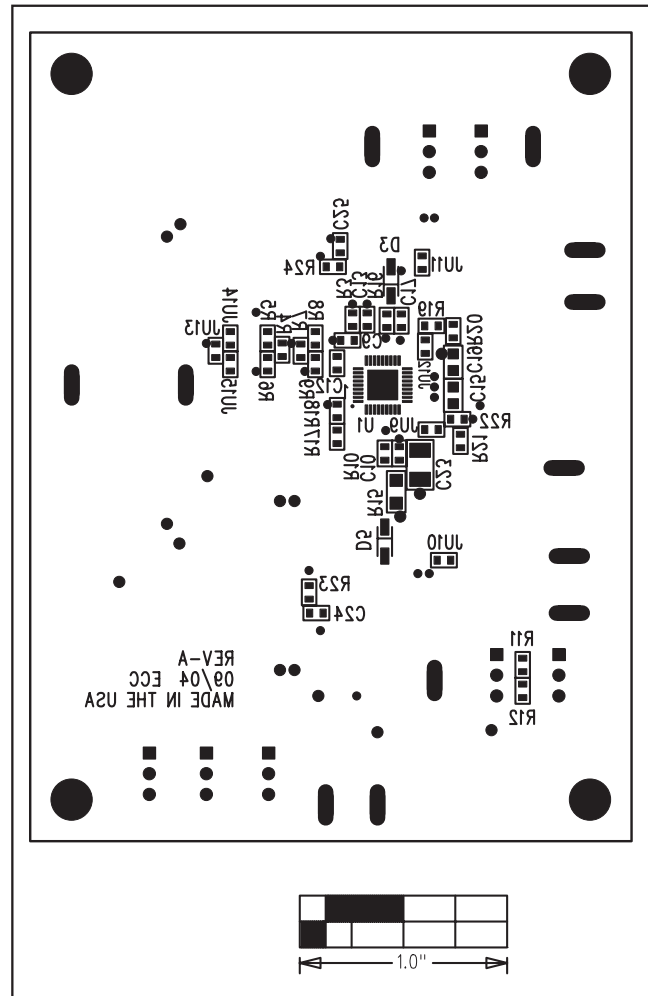
Figure 7. MAX1537 EV Kit Component Placement Guide—Solder Side
