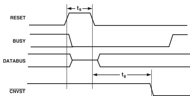
Figure 12. RESET Timing
