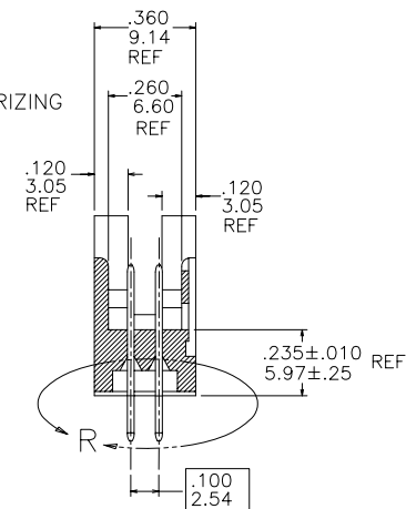
SECTION F-F
