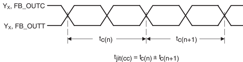
Figure 3. Cycle-to-Cycle Jitter
