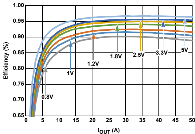
FIGURE 8. EFFICIENCY vs OUTPUT CURRENT AT V_{IN} = 9\text{V} , f_{SW} = 300\text{kHz} FOR VARIOUS OUTPUT VOLTAGES
