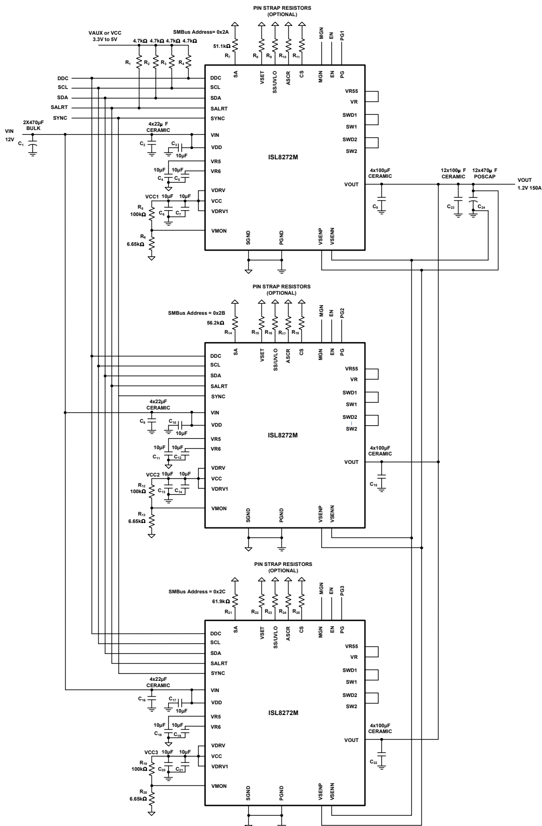
FIGURE 5. TYPICAL APPLICATION CIRCUIT - THREE MODULE CURRENT SHARING
