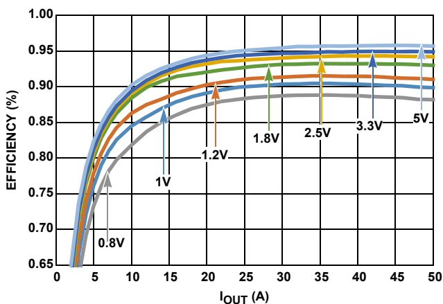
FIGURE 10. EFFICIENCY vs OUTPUT CURRENT AT V_{IN} = 12\text{V} , f_{SW} = 300\text{kHz} FOR VARIOUS OUTPUT VOLTAGES
