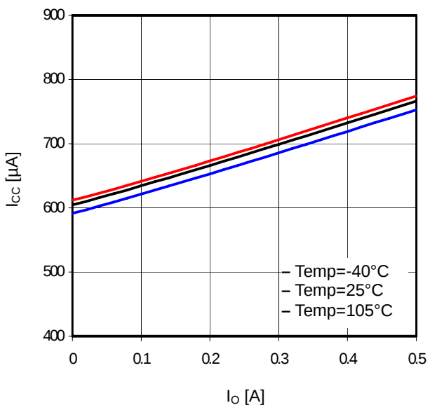
Figure 30. I_O-I_{CC}
