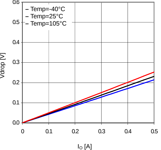
Figure 38. Minimum dropout Voltage 5 ( V_{CC}=12.0V )
