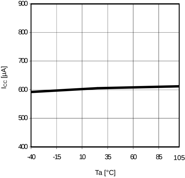
Figure 22. T_a - I_{cc}
