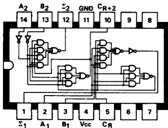
B61 SN7482N 2-bit binary full adder
