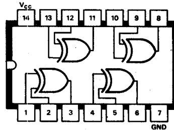
B65 SN7486N SN74S86N Quad 2-input exclusive-OR element
