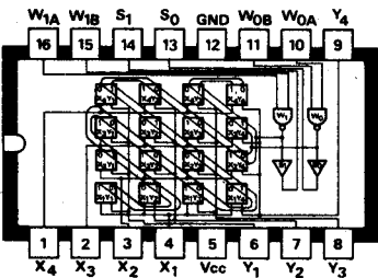
B63 SN7484N 16-bit read/write memory
