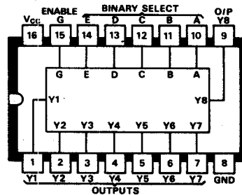
B66 SN7488N/AN 256-bit ROM (32 x 8)
