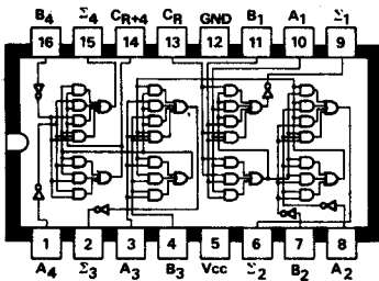
B62 SN7483N 4-bit binary full adder
