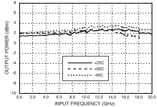
Output Power vs. Temperature, Pin = 0 dBm
