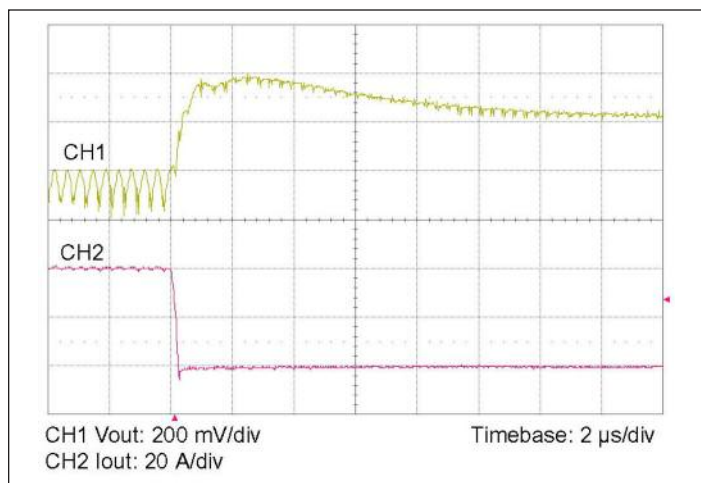
Figure 11 — 40 – 0 A load step with 100 \mu\text{F} input capacitor and no output capacitor.
