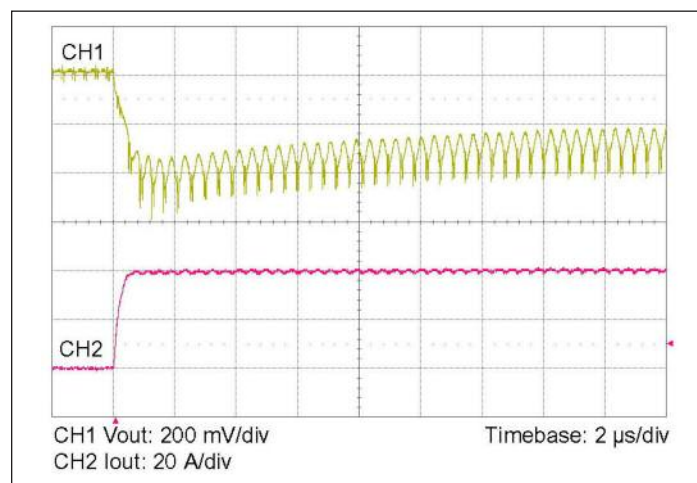
Figure 10 — 0 – 40 A load step with 100 \mu\text{F} input capacitor and no output capacitor.
