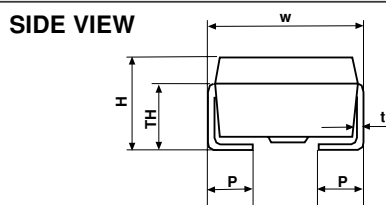
FIGURE 4 - DIMENSIONS AND IMPRINTING
