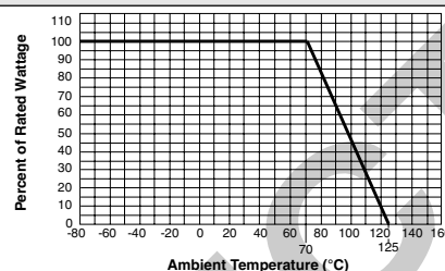
FIGURE 3 - POWER DERATING CURVE
