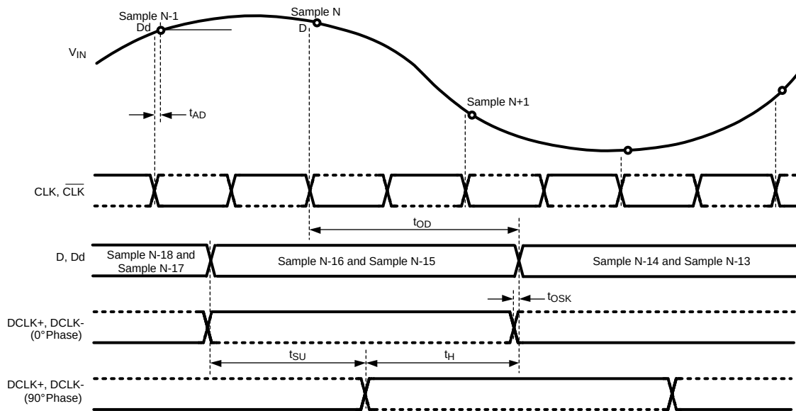
Figure 3. ADC081500 Timing — DDR Clcking
