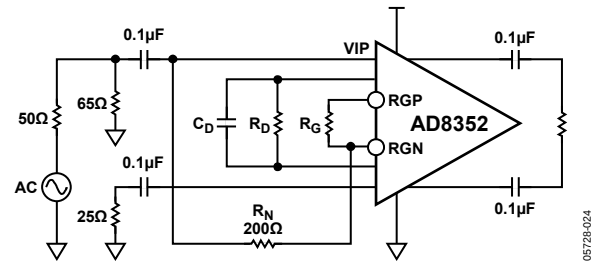
Figure 26. Single-Ended Schematic
