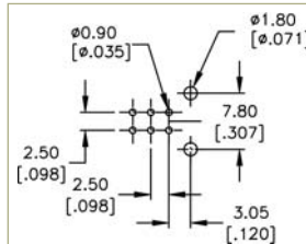
P.C. MOUNTING
