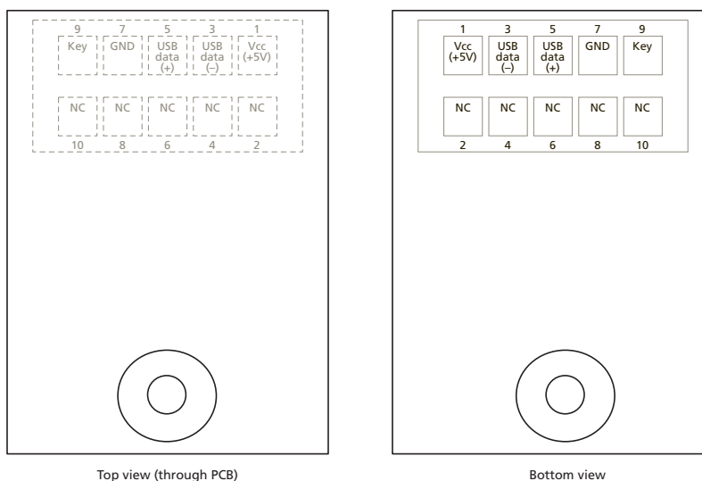
Figure 2: Pin Assignments: 2 x 5 Connector
