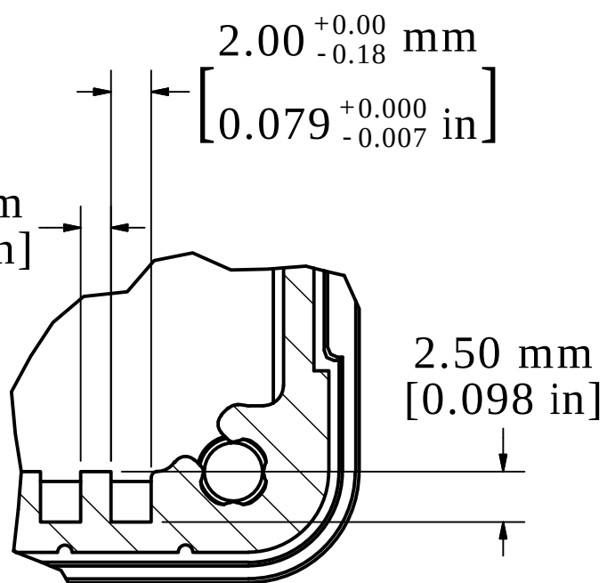
DETAIL W
