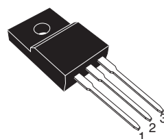
TO-220FPAB DMV1500MFD
