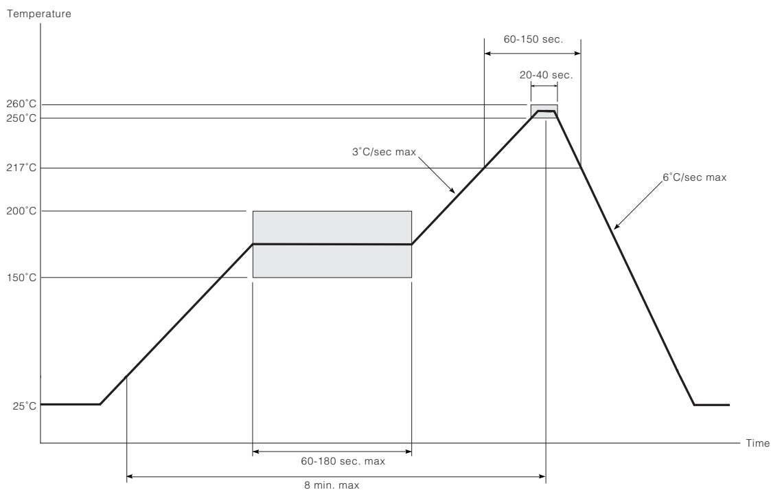
Figure 3-2: Pb-free Solder Reflow Profile (Applicable to Pb-free only)
