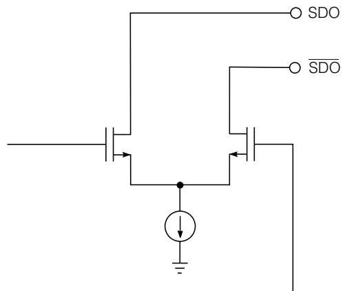
Figure 3-6: Serial Digital Output (GS1560A only)
