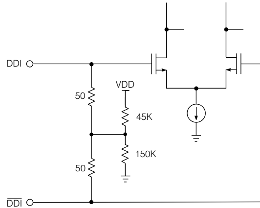
Figure 3-3: Serial Digital Input
