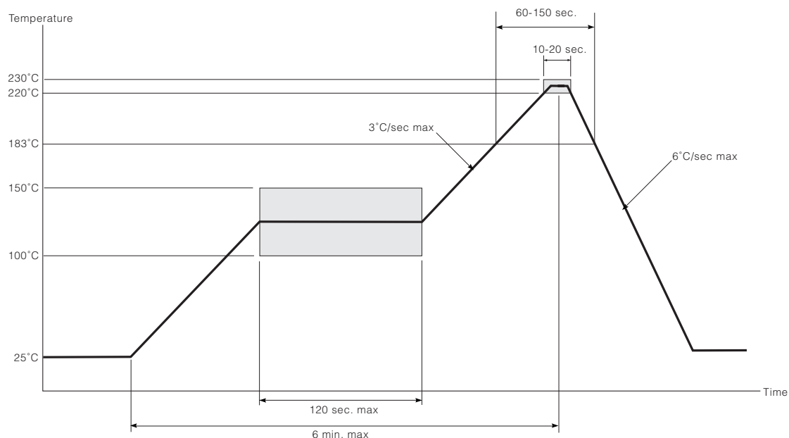
Figure 3-1: Conventional Solder Reflow Profile (Applicable to Pb-free and conventional packages)
