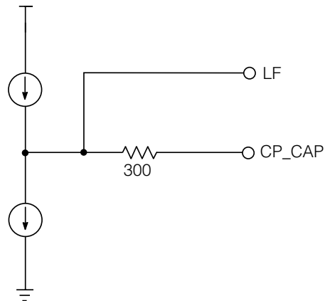
Figure 3-7: VCO Control Output & PLL Lock Time Capacitor
