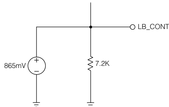
Figure 3-5: PLL Loop Bandwidth Control
