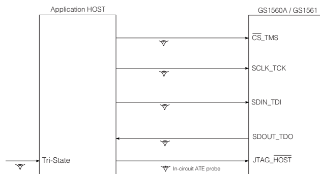
Figure 4-15: System JTAG
