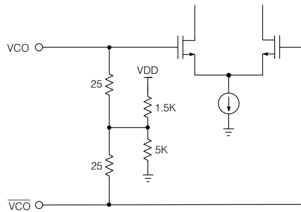
Figure 3-4: VCO Input
