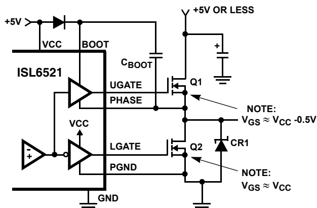
FIGURE 8. MOSFET GATE BIAS
