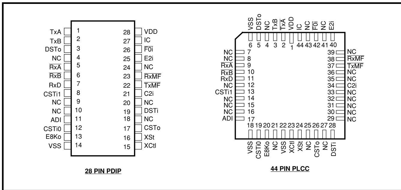
Figure 2 - Pin Connections
