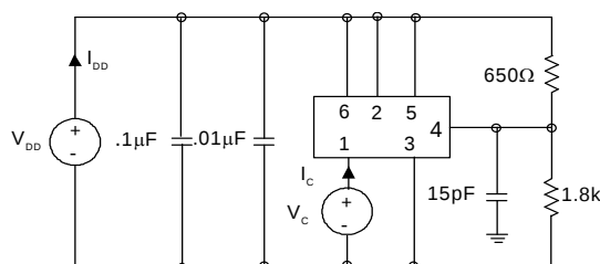
Figure 2. Typical Output Test Conditions (25 \pm 5°C)
