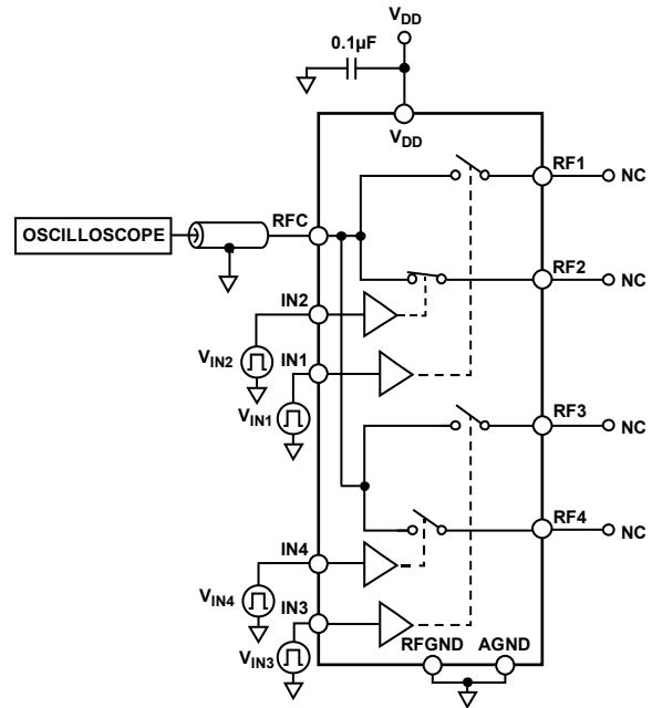
Figure 20. Video Feedthrough
