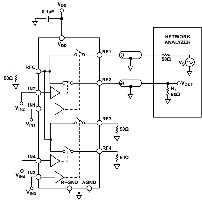
Figure 19. Crosstalk
