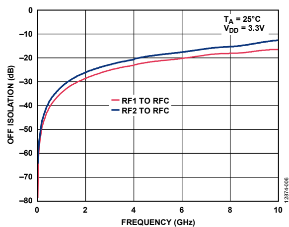
Figure 8. Off Isolation vs. Frequency ( V_{DD} = 3.3\text{ V} )
