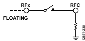
Figure 27. RFX Pins Left Open Circuit
