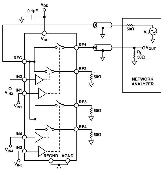
Figure 18. Isolation
