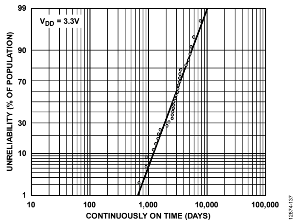
Figure 34. Continuously on Lifetime, V_{DD} = 3.3\text{ V} , 50°C, Sample Size 31 Parts
