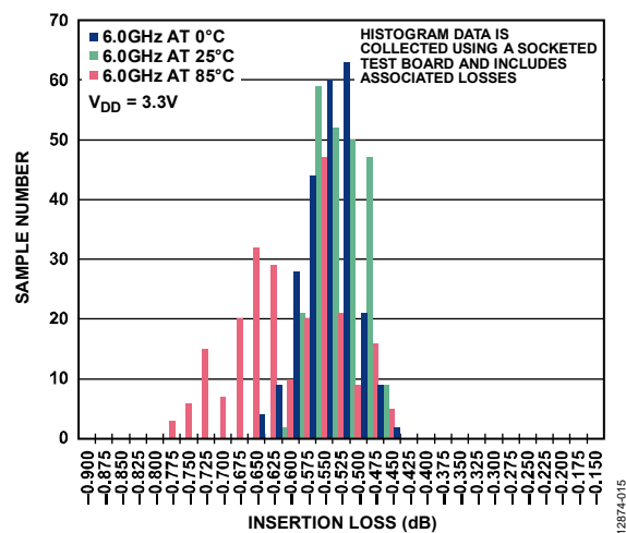
Figure 16. 6.0 GHz Insertion Loss Histogram vs. Temperature ( V_{DD} = 3.3 V )
