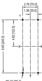
T7 3 POLE DRILLING FRONT VIEW
