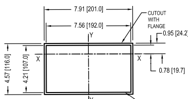
T7 3 & 4 POLE REDUCED CUTOUT FOR DOOR COMPARTMENT
