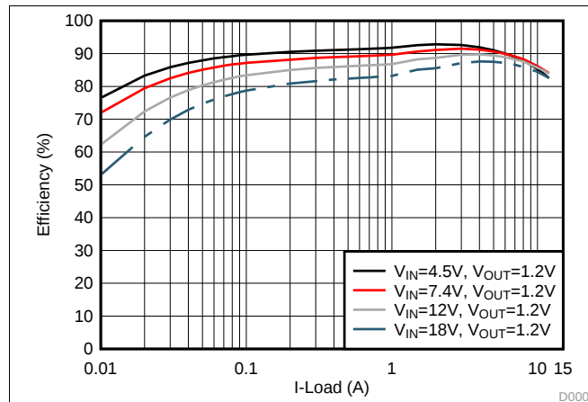
Figure 19. Efficiency Curve
