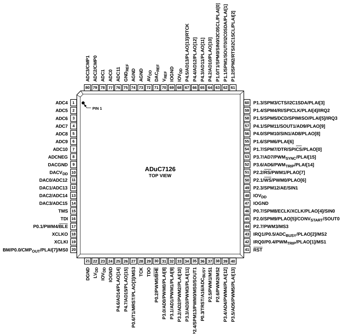
Figure 8. ADuC7126 Pin Configuration
