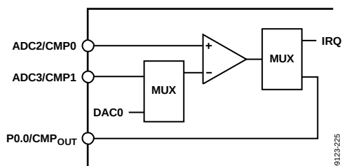
Figure 43. Comparator
