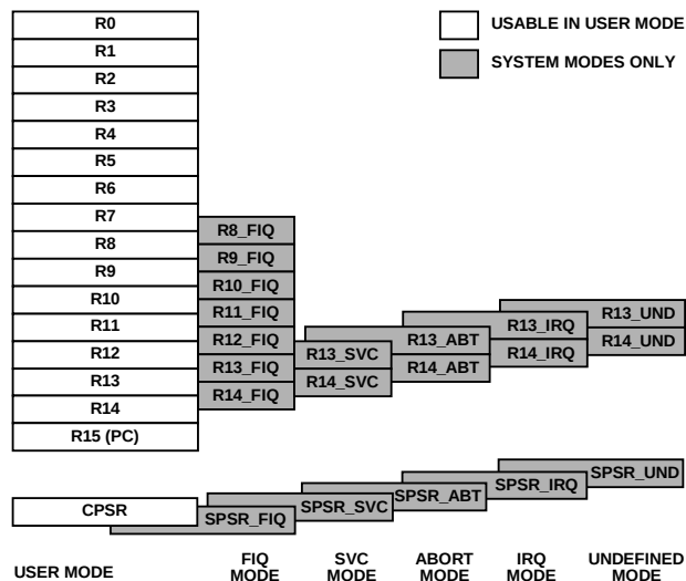
Figure 23. Register Organization
