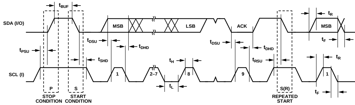
Figure 2. I²C-Compatible Interface Timing
