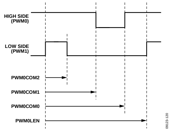
Figure 49. PWM Timing
